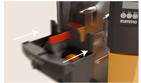
3. Fit the squeezing system
